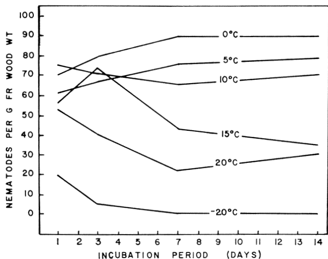
Figure 5.--Effect of low temperatures on pinewood nematode population development in southern pine chips.
