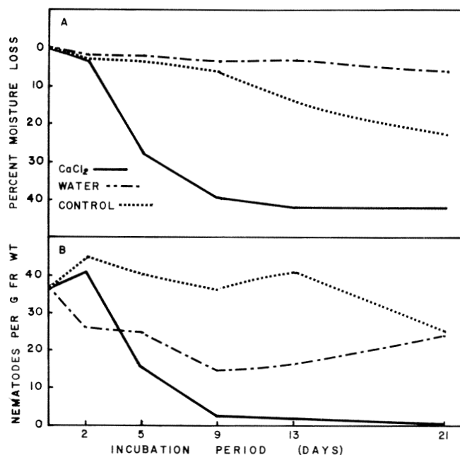
Figure 6.--Curves showing moisture loss in southern pine chips (A) and corresponding changes in population levels of pinewood nematode (B) at 35 °C over time.
