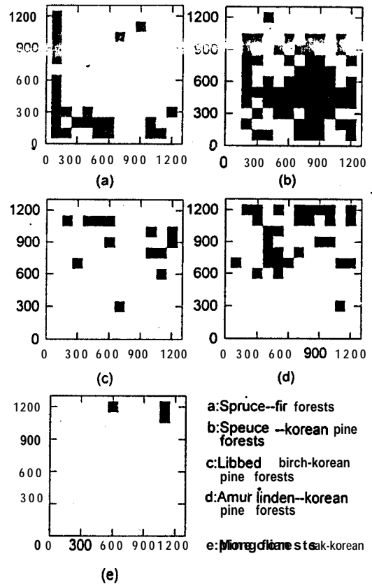
Fig. 5. Spatial distributions of forest types at landscape level in sampled region
