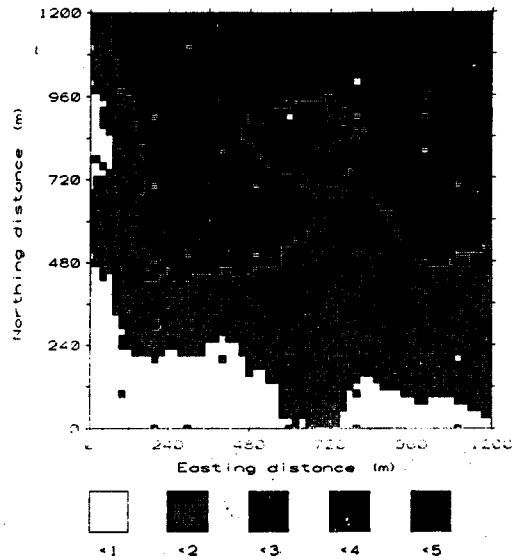
Fig. 4. A simulation of landscape pattern of old growth forest of Korean pine by block kriging.
