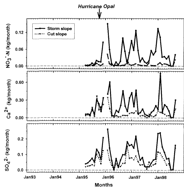
Figure 7. Modeled nutrient export from both the Storm hillslope (●) and the Cut hillslope (▽).
