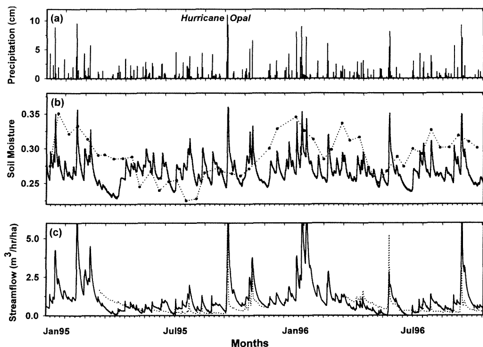
Figure 3. Rainfall, soil moisture, and hillslope run-off dynamics for the Storm hillslope. For the 22-month period bracketing Hurricane Opal, the panels show: a daily rainfall, b modeled and measured soil moisture, and c measured WS 56 streamflow and modeled hillslope water outflow. On b and c, the solid lines represent the modeled data, and the dotted lines represent the measured data.
