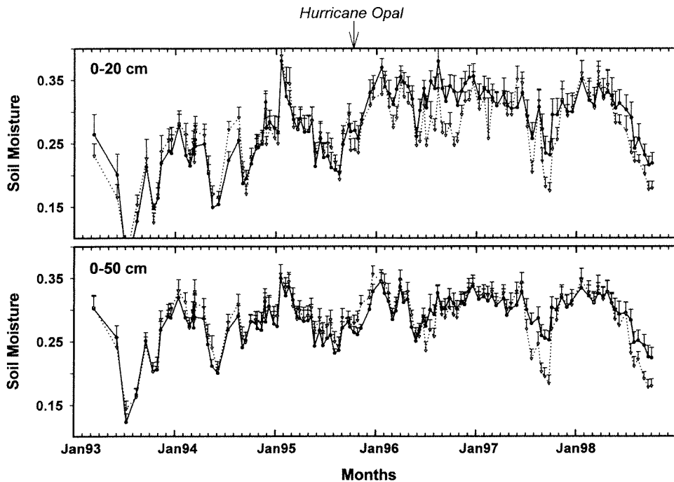
Figure 4. Soil moisture dynamics at 0–20 cm and 0–50 cm on the Cut and Storm hillslopes. The plots compare mean soil moisture, with error bars showing 1 SE, within 5 m of the stream at two different depths for the Cut hillslope ( \nabla ) and the Storm hillslope ( \bullet ).
