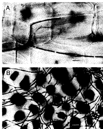
Fig. 1. Endophytic hyphae in (A) leaf sheath and (B) aleurone seed tissue of Lolium perenne (PI 205278). Scale bar = 5 \mu\text{m} .
