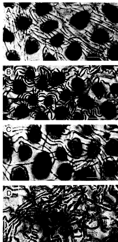
Fig. 2. Comparative morphology of endophytic hyphae in aleurone seed tissues of (A) Lolium multiflorum (PI 410154), (B) L. persicum (PI 222807), (C) L. rigidum (PI 250805), and (D) L. temulentum (PI 249725). Scale bar = 5 \mu\text{m} .
