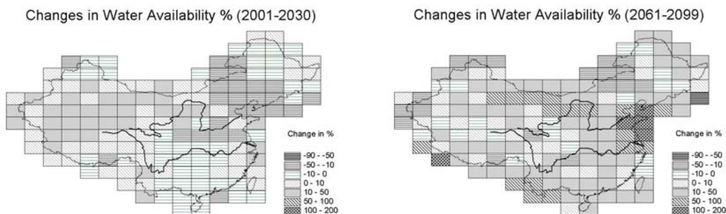
Figure 3. Predicted Changes in Water Availability for the Next 30 and 100 Years.
