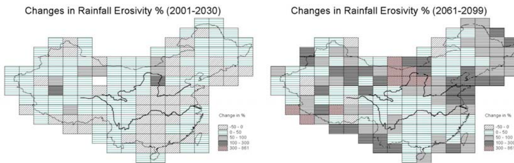
Figure 2. Predicted Changes in Rainfall Erosivity for the Next 30 and 100 Years.
