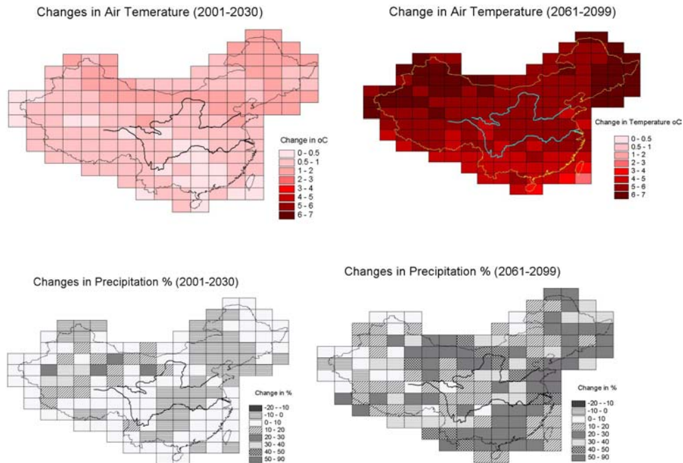
Figure 1. Climate Change Scenarios Predicted by the HadCM3 SRES GCM.
