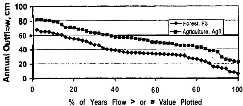
Figure 10. Frequency of predicted annual outflows (subsurface drainage + surface RO) for the forested and agricultural sites.
