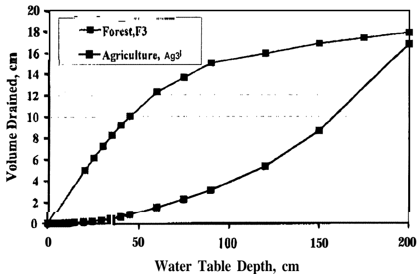
Figure 7. Relationship between volume of water drained (per unit surface area) and water table depth. The volume (or depth) drained is the amount of water that would have to be removed to lower the water table from the surface to the depth on the abscissa.
