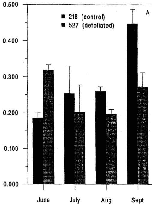
FIGURE 2. Throughfall inputs (avg. mg/l NO 3 -N) on study sites 218 (control) and 527 (defoliated). A = 1997, B = 1998.
