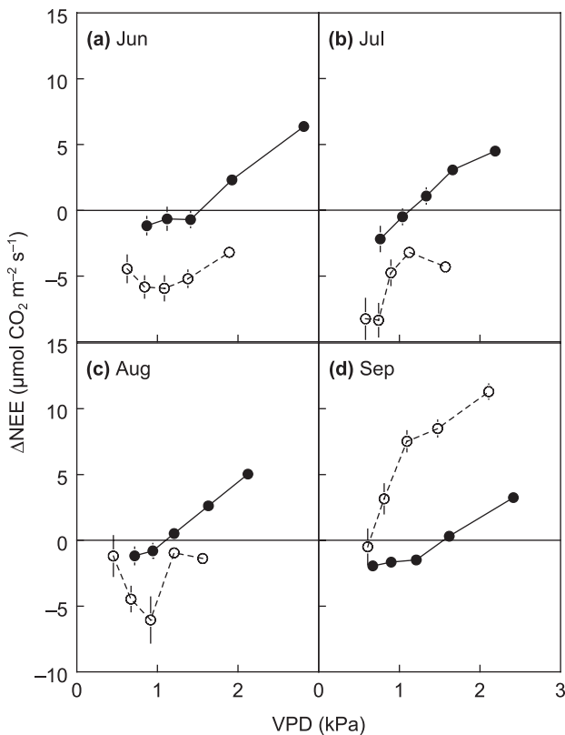
Fig. 7 Response of photosynthetically active radiation (PAR)-normalized net ecosystem exchange (NEE) of carbon to vapor pressure deficit (VPD) at midday (12:00–13:00 CDT; mean \pm SE, each group during the same month in the same year has the same number of observations). 2004, open circles; 2005, closed circles. The dependence of NEE on PAR in low-VPD conditions was calculated from data with VPD below the median using Eqn 1. The figure shows the difference between observed and modeled values for the upper 50% of the data. Positive values indicate VPD-induced suppression of the magnitude of NEE.
