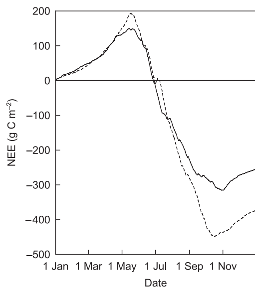
Fig. 2 Yearly cumulative net ecosystem exchange (NEE) of carbon in an oak woodland in Ohio, USA, in 2004 (dashed line) and 2005 (solid line).
