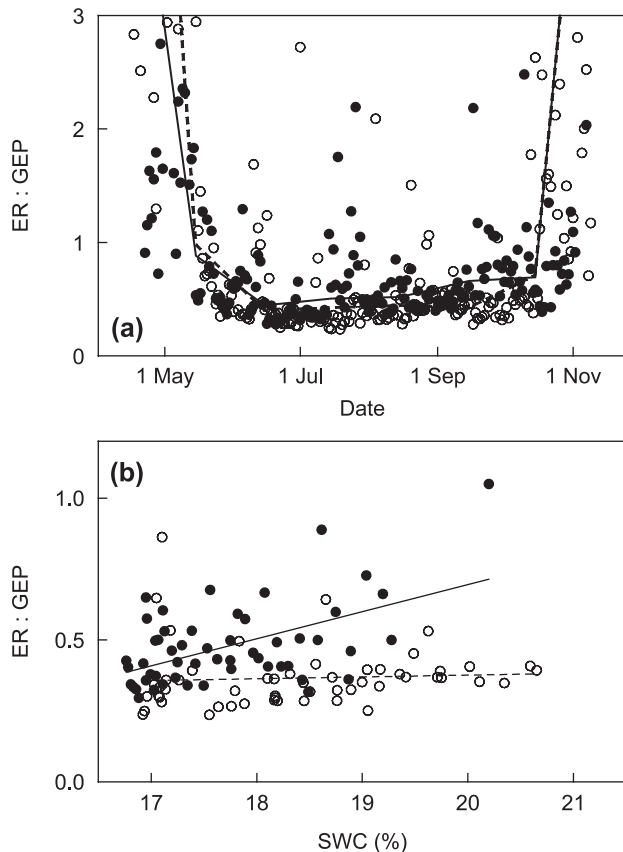
Fig. 5 The seasonal dynamics of the daily cumulative ecosystem respiration (ER) : gross ecosystem productivity (GEP) ratio and the ratios of monthly totals (a), and the dependence of the daily ratio on daily mean soil water content (SWC) during nonrainy days during the growing season (b). 2004, open circles; 2005, closed circles.
