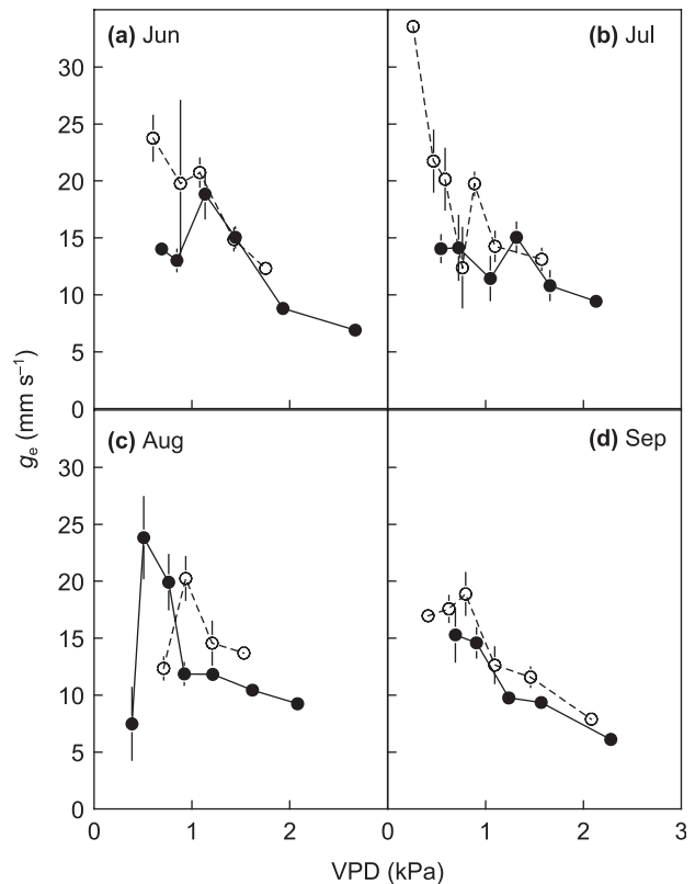
Fig. 6 Comparison of the dependence of canopy conductance ( g_c ) on vapor pressure deficit (VPD) at midday (12:00–13:00 central daylight time (CDT); mean \pm SE, each group during the same month in the same year has the same number of observations) between the two years (2004, open circles; 2005, closed circles) in an oak woodland in Ohio, USA.
