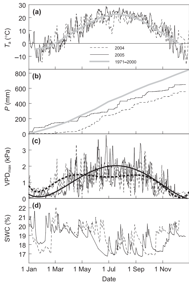
Fig. 1 Temporal dynamics of daily mean and monthly normal air temperatures ( T_a ) (a), daily cumulative measured and monthly cumulative normal precipitation ( P ) (b), daily maximum vapor pressure deficit ( \text{VPD}_{\text{max}} ) (c) and daily mean soil water content (SWC) (d) in an oak woodland in Ohio, USA, during 2004 and 2005. The curves fitted to \text{VPD}_{\text{max}} are best-fit sixth-degree polynomials to highlight seasonal trends. The 30-yr mean indicators are from National Climatic Data Center ( http://www.ncdc.noaa.gov/oa/ncdc.html ).
