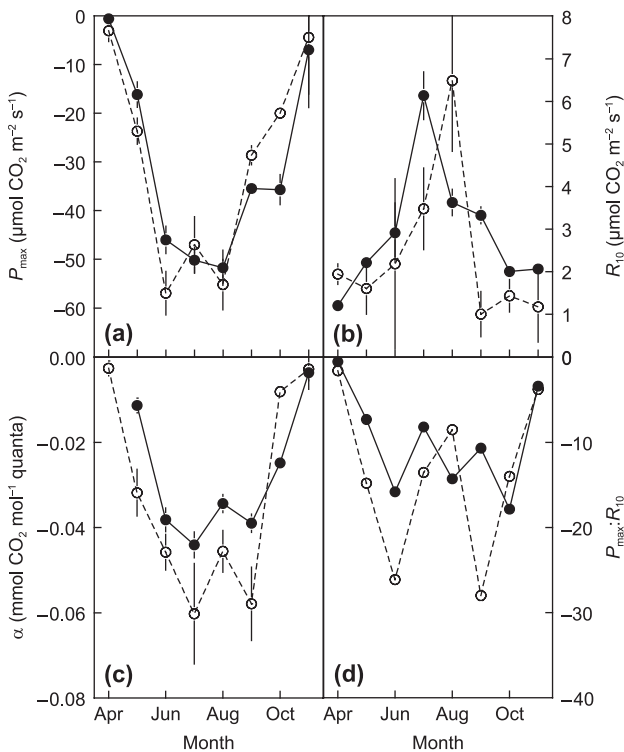
Fig. 3 Monthly canopy maximum photosynthetic capacity ( P_{max} ) (a), reference respiration ( R_{10} ) (b), apparent quantum yield ( \alpha ) (c), and the ratio of P_{max} and R_{10} during the two years of study (2004, open circles; 2005, closed circles). Error bars represent 1 SE of the parameter estimate.
