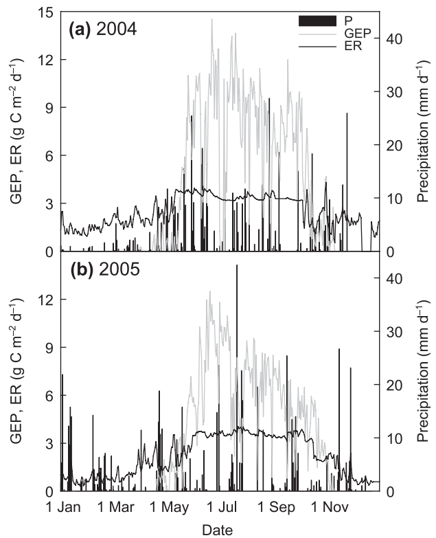
Fig. 4 Daily gross ecosystem productivity (GEP), ecosystem respiration and daily total precipitation ( P ) in a nondrought year, 2004 (a), and a drought year, 2005 (b). Larger rain events suppress GEP and stimulate ecosystem respiration (ER).
