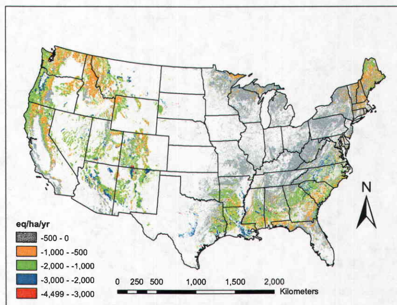
Fig. 3. Average annual critical leaching of forest soil acid neutralizing capacity expressed in \text{eq ha}^{-1} \text{yr}^{-1} for the conterminous US for the years 1994–2000 at a 1\text{-km}^2 spatial resolution.
