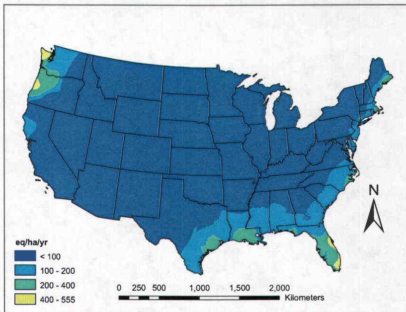
Fig. 6. Average annual wet chloride deposition expressed in \text{eq ha}^{-1} \text{yr}^{-1} for the conterminous US for the years 1994–2000 at a 1\text{-km}^2 spatial resolution.
