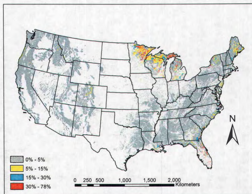
Fig. 1. Forest soil percent organic matter concentration averaged to a depth of 1.52 m for the conterminous US at a 1\text{-km}^2 spatial resolution.
