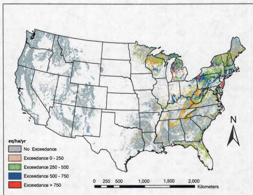
Fig. 8. Average annual exceedance of the critical acid load for forest soils expressed in \text{eq ha}^{-1} \text{yr}^{-1} for the conterminous US for the years 1994–2000 at a 1\text{-km}^2 spatial resolution.
