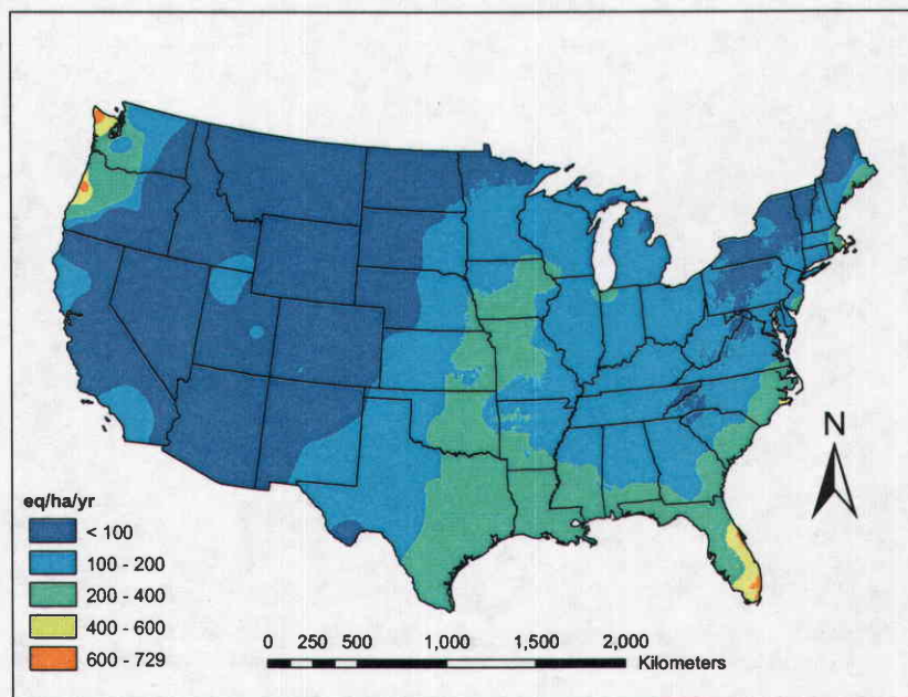
Fig. 5. Average annual base cation deposition expressed in \text{eq ha}^{-1} \text{yr}^{-1} for the conterminous US for the years 1994–2000 at a 1\text{-km}^2 spatial resolution.
