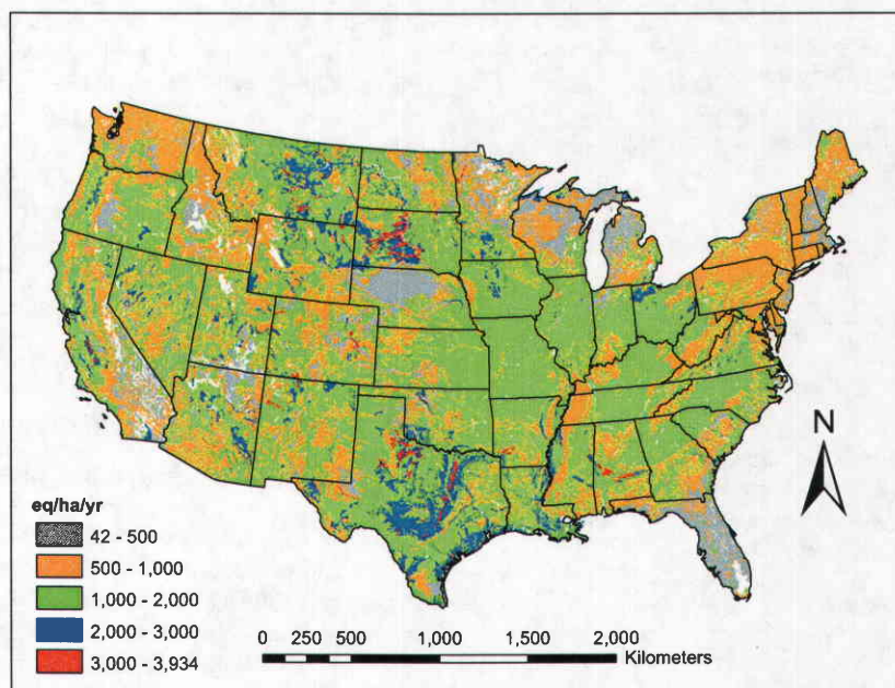
Fig. 2. Average annual forest soil base cation weathering expressed in \text{eq ha}^{-1} \text{yr}^{-1} for the conterminous US for the years 1994–2000 at a 1\text{-km}^2 spatial resolution.
