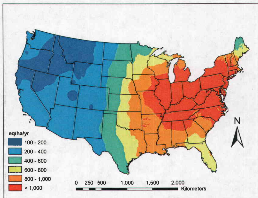
Fig. 4. Average annual combined wet and dry nitrogen and sulfur deposition expressed in \text{eq ha}^{-1} \text{yr}^{-1} for the conterminous US for the years 1994–2000 at a 1\text{-km}^2 spatial resolution.
