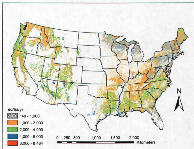
Fig. 7. Average annual critical acid load for forest soils expressed in \text{eq ha}^{-1} \text{yr}^{-1} for the conterminous US for the years 1994–2000 at a 1\text{-km}^2 spatial resolution.
