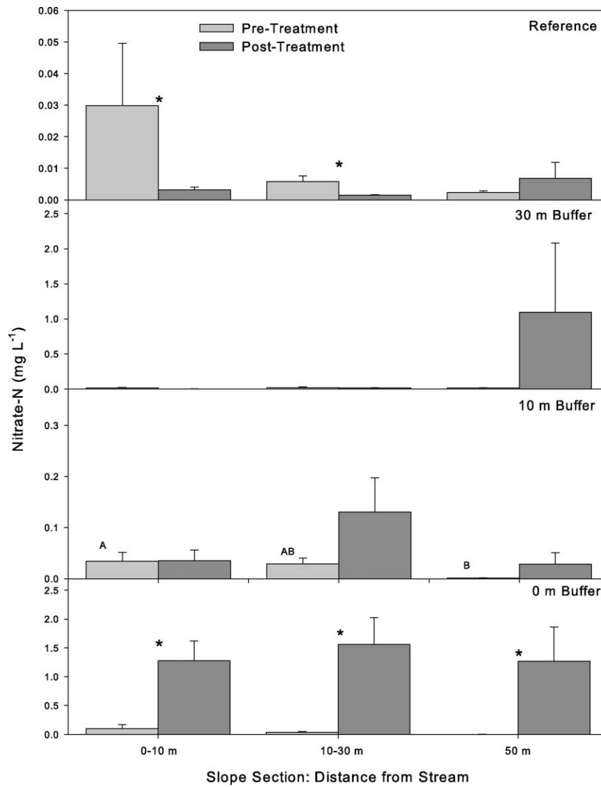
Fig. 8. Deep soil (lower B horizon) solution \text{NO}_3^- -N concentrations collected using soil porous cup, tension lysimeters. Site values presented are means of seasonal mean values of monthly composited samples for each transect at each slope position. Bars represent one standard error of the mean. "*" designates significant differences between pre- and post-treatment values for a slope sections within a site. Letters (A, B, C) designate significant differences between slope sections within a site.
