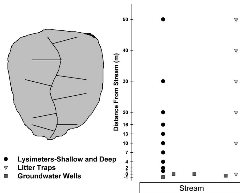
Fig. 1. Graphic depiction of site transect layout along the 200 m stream reach. Nutrient cycling transects are centered on litter fall traps, with tension lysimeters off-set from transect center-line by 7.5 m. Groundwater wells are located between the end of the transect and the center of the stream. Soil sample collections take place at randomly selected location along the sample line.
