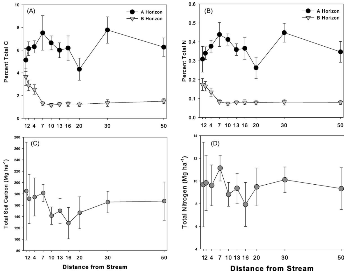
Fig. 2. Total C and N through the soil profile along the transect for near-stream to upper-slope position. Data represent the mean value of pre-harvest soil collection from all four sites ( n = 4 ) at each distance from the stream. Error bars represent one standard error of the mean. (A) Carbon concentration (%) in the A and the B horizon soils. (B) Nitrogen concentration (%) in the A and B horizon soils. (C) Total C in the soil profile \text{Mg ha}^{-1} from soil surface to surface of the saprolite. (D) Total C in the soil profile \text{Mg ha}^{-1} from soil surface to surface of the saprolite.
