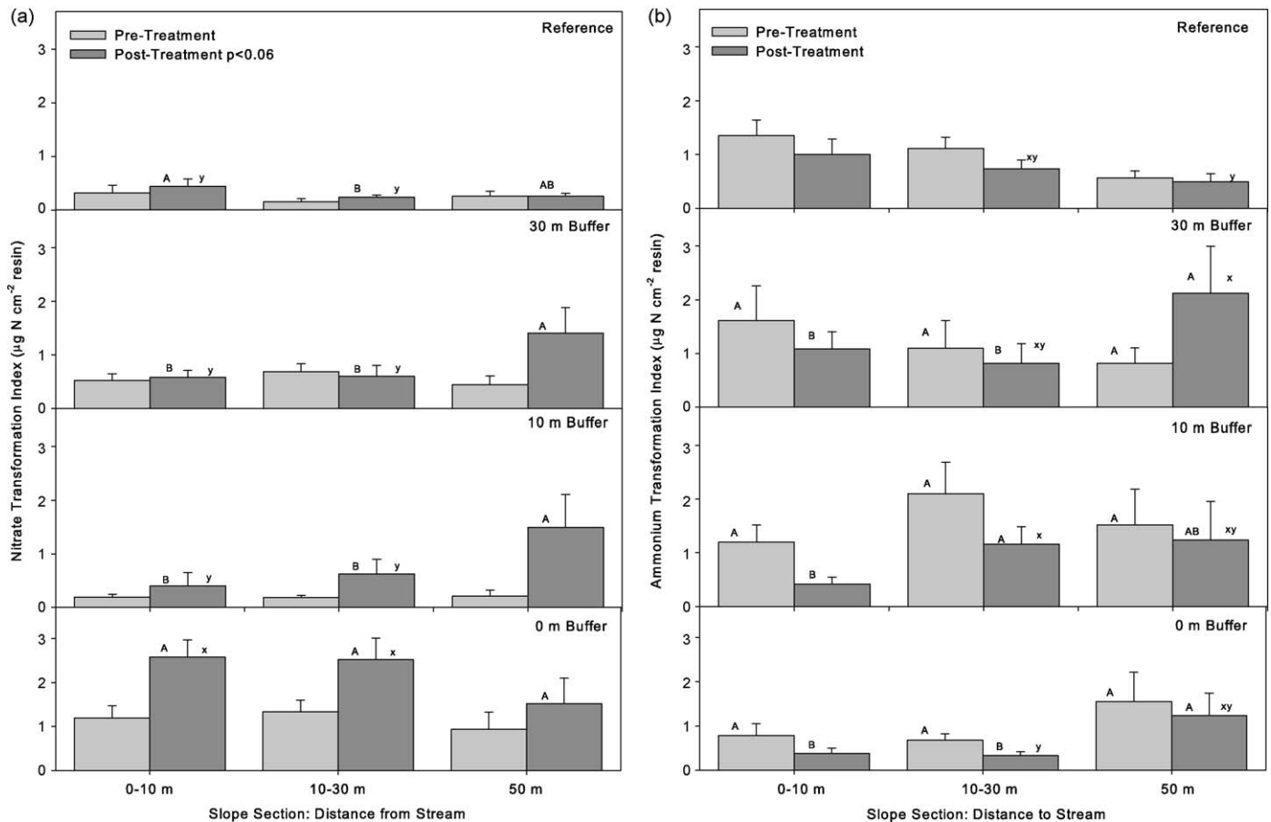
Fig. 6. (a) Index of soil nitrification potential as measured using \text{NO}_3^- -N captured during a 14 day on anion exchange resin sheets, pre- and post-treatment in the reference, 30 m buffer, 10 m buffer, and 0 m buffer sites along the slope including near-stream, mid-slope, and upper-slope positions. Post-treatment data shown are the means spring, summer and fall collections, of each sample transect ( n = 4 ) for each slope section. Bars represent one standard error of the mean. Bars within a site with different letters (A, B, C) designate significant differences among slope sections within a site. Bars within a slope section with different letters (x, y, z) designate significant differences for a slope section between sites. (b) Index of soil N mineralization potential as measured using \text{NH}_4^+ -N captured during a 14 day on cation exchange resin sheets, pre- and post-treatment in the reference, 30 m, 10 m, and 0 m buffer sites along the slope including near-stream, mid-slope, and upper-slope positions. Post-treatment data shown are the means spring, summer and fall collections, of each sample transect ( n = 4 ) for each slope section. Bars represent one standard error of the mean. Bars within a site with different letters (A, B, C) designate significant differences among slope sections within a site. Bars within a slope section with different letters (x, y, z) designate significant differences for a slope section between sites.
