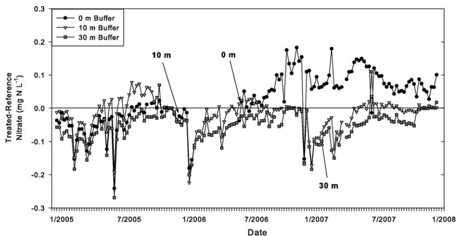
Fig. 9. Stream \text{NO}_3^- -N concentrations response to forest harvest for each of the three riparian zone buffer widths. Stream samples are collected weekly below the harvested area and reference. Values shown are treated minus reference for weekly concentrations, collections began in January 2005. An arrow indicates beginning of post-harvest sample collection for each site.
