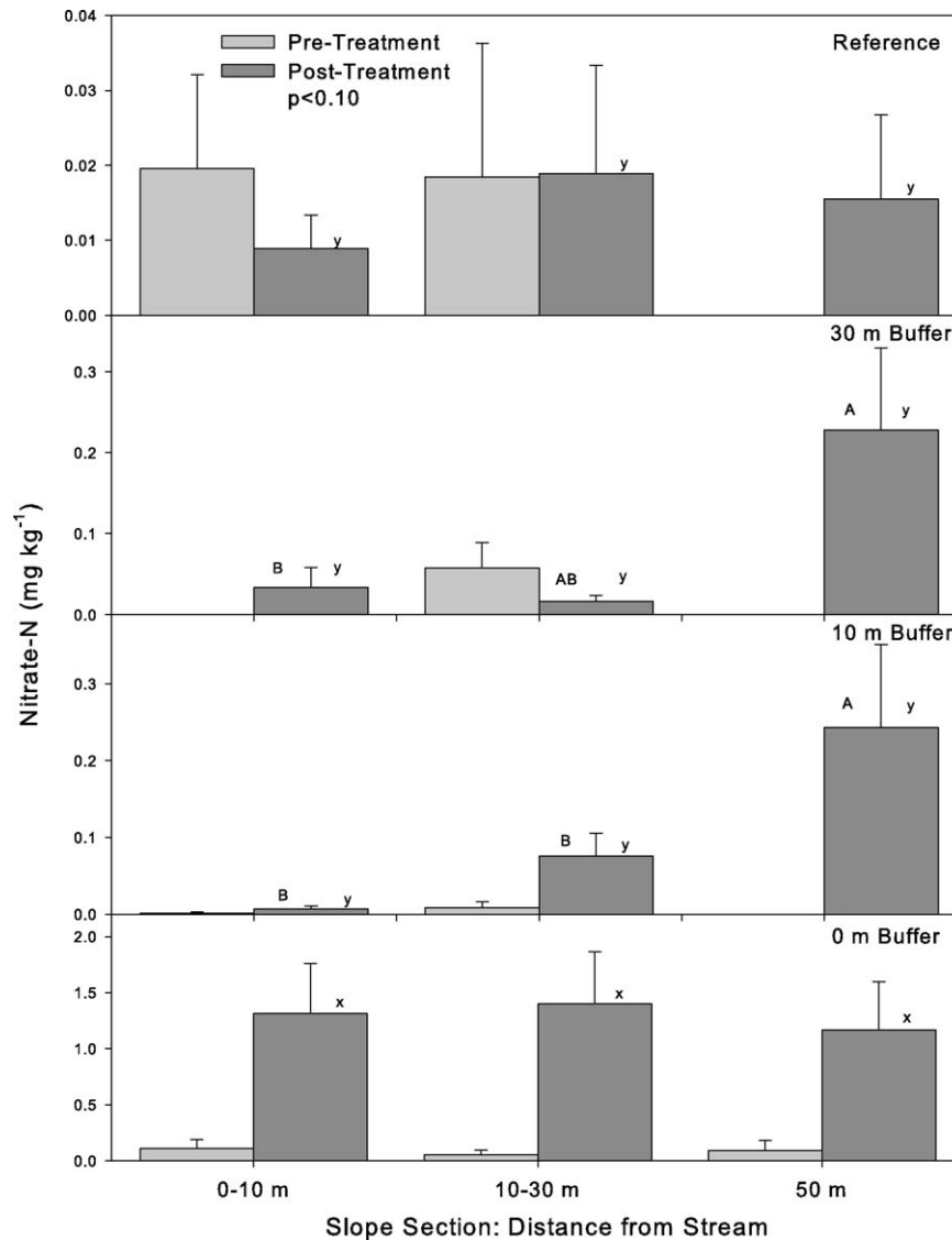
Fig. 4. Soil \text{NO}_3^- -N concentration in surface soils (0–10 cm), pre- and post-treatment in the reference, 30 m buffer, 10 m buffer, and 0 m buffer sites along the slope including near-stream, mid-slope, and upper-slope positions. Post-treatment data shown are the mean values of spring, summer and fall collections, of each sample transect ( n = 4 ) for each slope section. Error bars represent one standard error of the mean. Bars within a site with different letters (A, B, C) designate significant differences among slope sections within a site. Bars within a slope section with different letters (x, y, z) designate significant differences for a slope section between sites.
