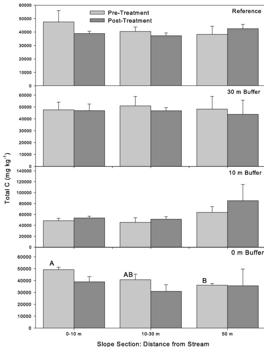
Fig. 3. Total soil C concentration in surface soils (0–10 cm), pre- and post-treatment in the reference, 30 m buffer, 10 m buffer, and 0 m buffer sites along the slope including near-stream, mid-slope, and upper-slope positions. Post-treatment data are the mean values of the first soil sample collection; of each sample transect ( n = 4 ) for each slope section. Error bars represent one standard error of the mean. Bars within a site with different letters (A, B, C) designate significant differences among slope sections within a site. Bars within a slope section with different letters (x, y, z) designate significant differences for a slope section between sites.
