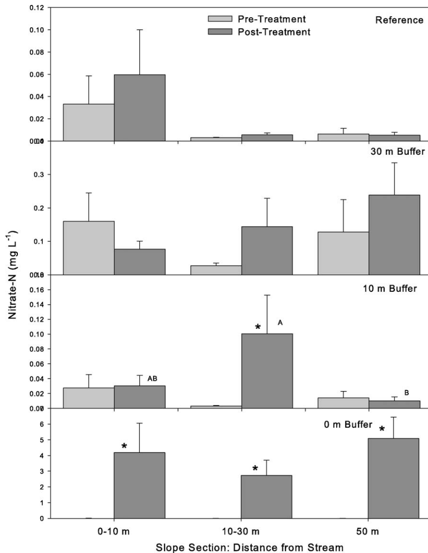
Fig. 7. Shallow soil (15 cm) solution \text{NO}_3^- -N concentrations collected using soil porous cup, tension lysimeters. Site values presented are means of seasonal mean values of monthly composited samples for each transect at each slope position. Bars represent one standard error of the mean. "*" designates significant differences between pre- and post-treatment values for a slope sections within a site. Letters (A, B, C) designate significant differences between slope sections within a site.
