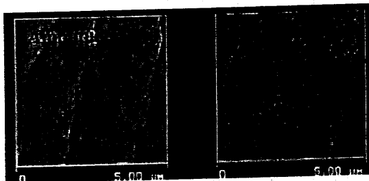
Figure 5 Amplitude and phase AFM analysis of 8.75% lignin pine kraft test sheets treated with 0.0 or 2.5% PLA and hot-pressed (press Conditions: 130°C, 2.30 \times 10^5 kPa, and 5 min).
