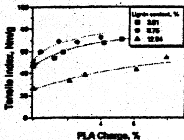
Figure 3 Analysis of PLA addition to pine kraft pulp test sheets prepared with different levels of residual lignin at a press temperature of 130°C and a press pressure of 2.30 \times 10^5 kPa for 5 min.
