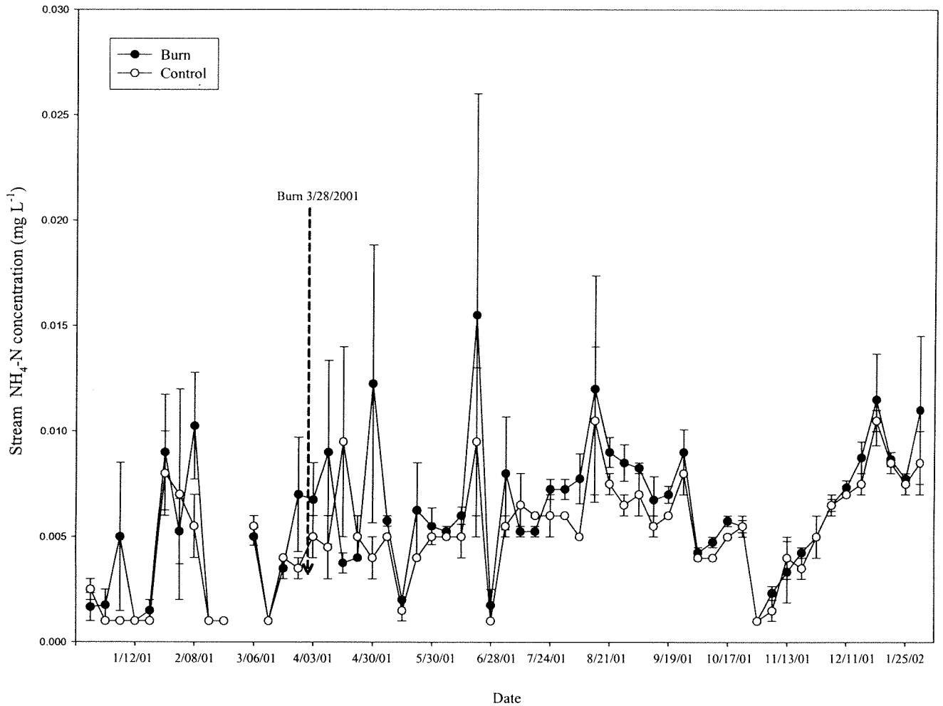
Figure 6. Stream ammonium-nitrogen ( \text{NH}_4^+\text{-N} ) concentrations collected from burn and control treatment sites from Jan. 2001 through Jan. 2002 in the Conasauga River Watershed in southeastern Tennessee and northern Georgia. Values are weekly means with standard error bars.
