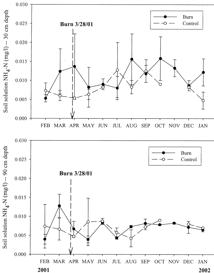
Figure 4. Soil solution ammonium-nitrogen (NH 4 + -N) concentrations at: (a) 30 cm and (b) 90 cm soil depths for burn and control treatment sites from Feb. 2001 to Jan. 2002 in the Conasauga River Watershed in southeastern Tennessee and northern Georgia. Values are monthly means with standard error bars.
