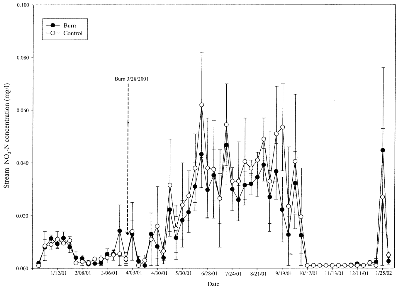
Figure 5. Stream nitrate-nitrogen ( \text{NO}_3^- -N) concentrations collected from burn and control treatment sites from Jan. 2001 through Jan. 2002 in the Conasauga River Watershed in southeastern Tennessee and northern Georgia. Values are weekly means with standard error bars.
