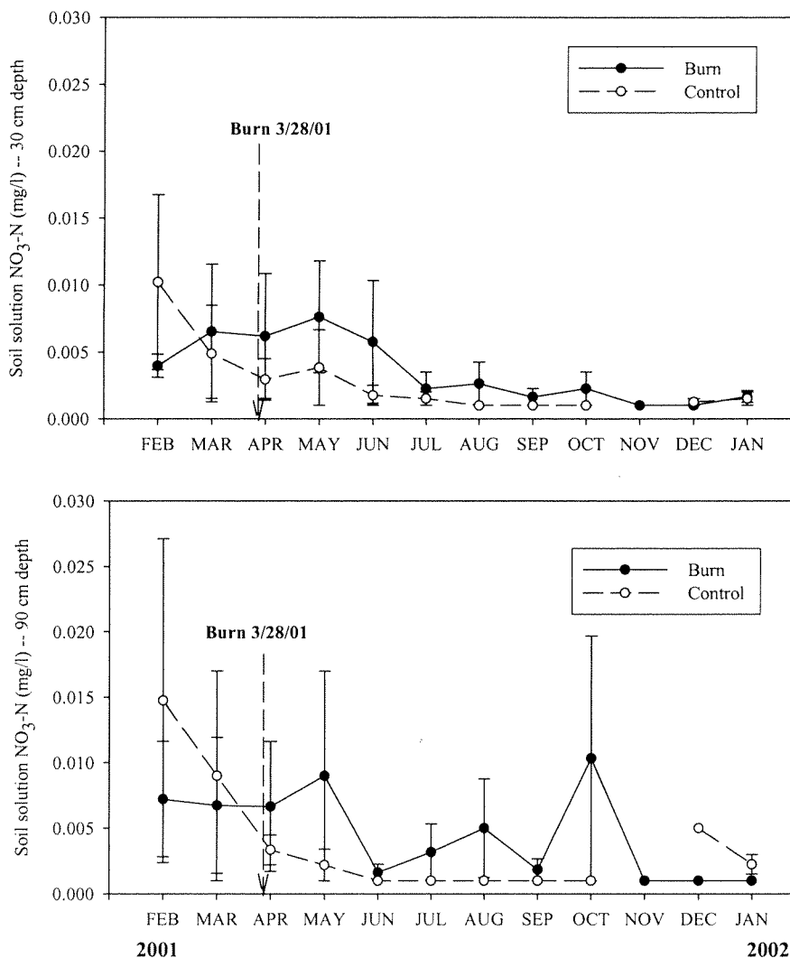
Figure 3. Soil solution nitrate-nitrogen ( \text{NO}_3^- -N) concentrations at: (a) 30 cm and (b) 90 cm soil depths for burn and control treatment sites from Feb. 2001 to Jan. 2002 in the Conasauga River Watershed in southeastern Tennessee and northern Georgia. Values are monthly means with standard error bars.
