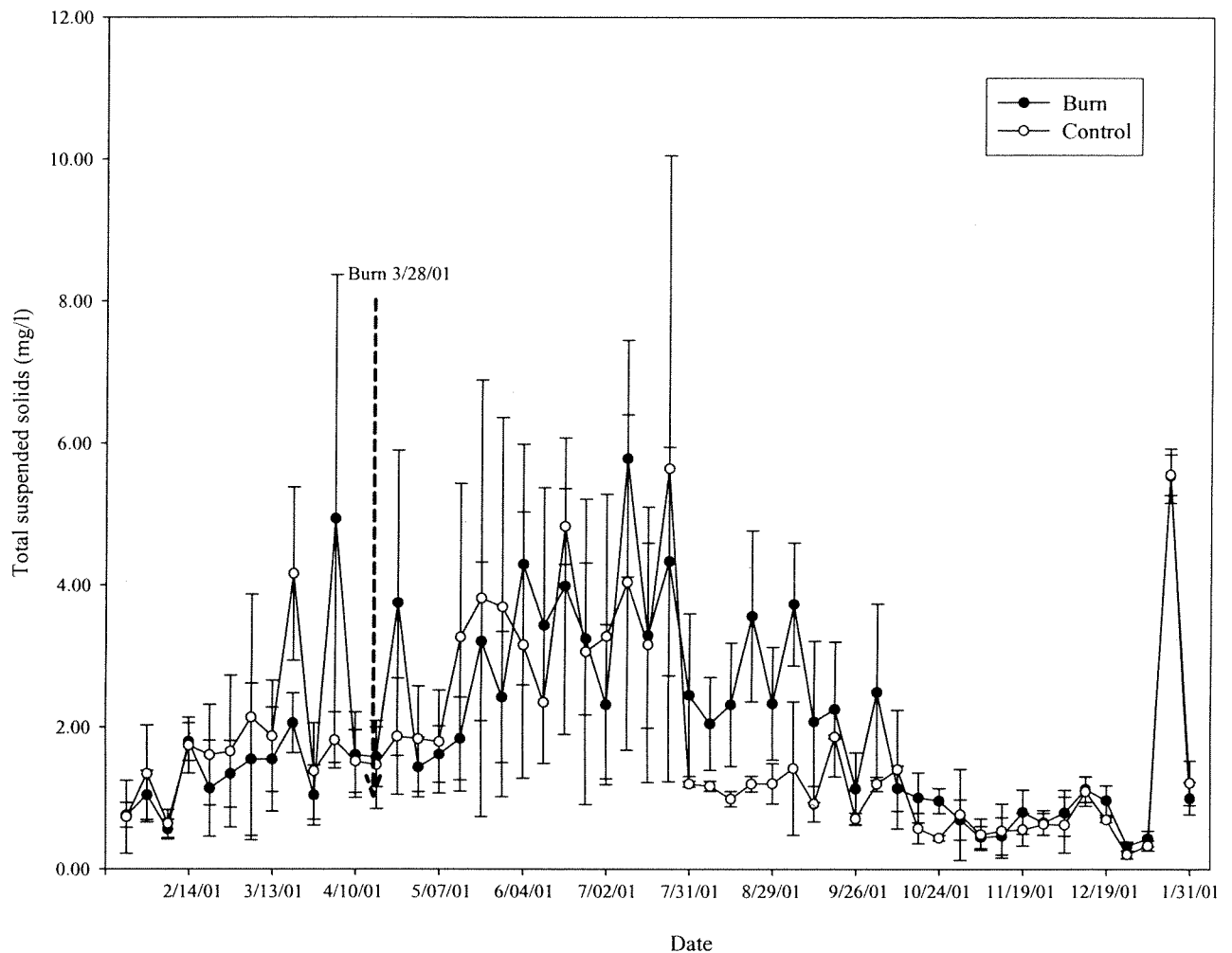
Figure 7. Stream total suspended solid (TSS) concentrations collected from burn and control treatment sites from Jan. 2001 through Jan. 2002 in the Conasauga River Watershed in southeastern Tennessee and northern Georgia. Values are weekly means with standard error bars.
