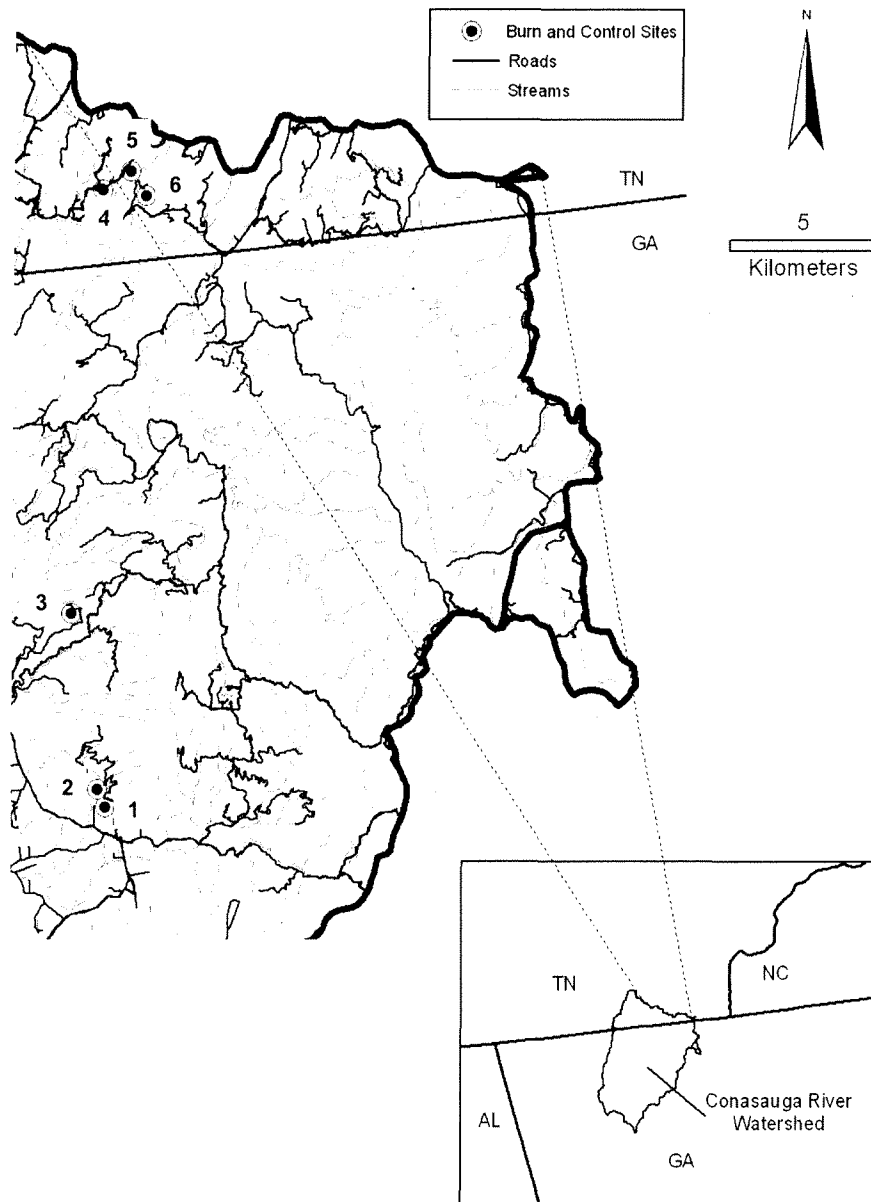
Figure 1. Map locations of the six subwatershed sites in the Conasauga River Watershed in southeastern Tennessee and northern Georgia. Site numbers are: 1, Muskrat Branch Burn; 2, Muskrat Branch Control; 3, Cohutta Springs Burn; 4, Sawmill Branch Burn; 5, Sawmill Branch Control; and 6, Halfway Branch Burn (adapted from Riedel and Vose 2002).
