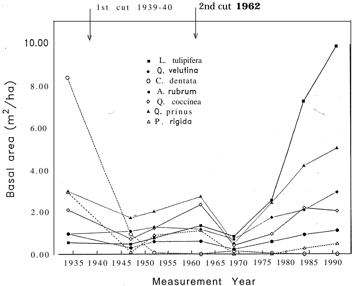
Fig. 2. Basal area of selected tree species in Watershed 13, Coweeta Basin from 1934 to 1991.
