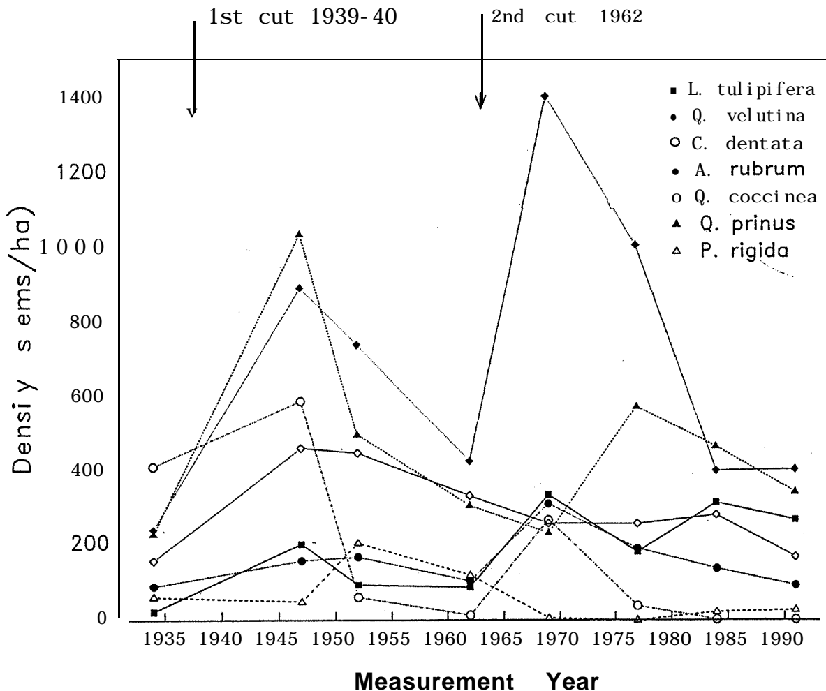
Fig. 1. Density of selected tree species in Watershed 13, Coweeta Basin from 1934 to 1991.
