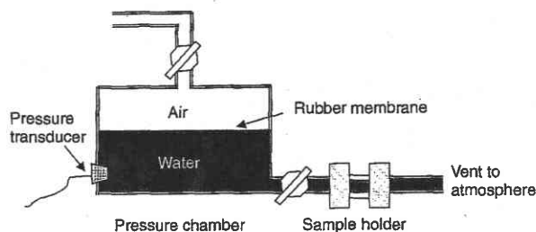
Figure 2. Diagram of the pressurized chamber apparatus used to measure conductivity under non-steady pressure gradients.
