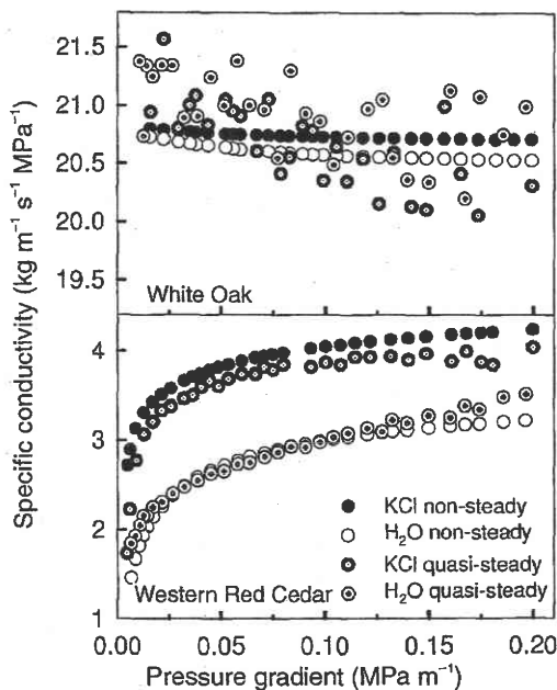
Figure 5. Specific conductivities of stem xylem in relation to non-steady and quasi-steady pressure gradients measured with the pressurized chamber using either 25 mmol KCl or deionized water as the perfusion fluid.
