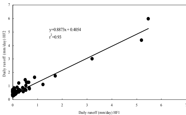
Figure 2. Daily runoff relationship in paired watersheds (HF1 and HF2) during calibration period, Hill Forest.
