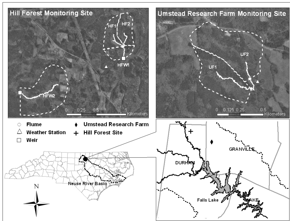
Figure 1. Watershed, weir and flume locations.
