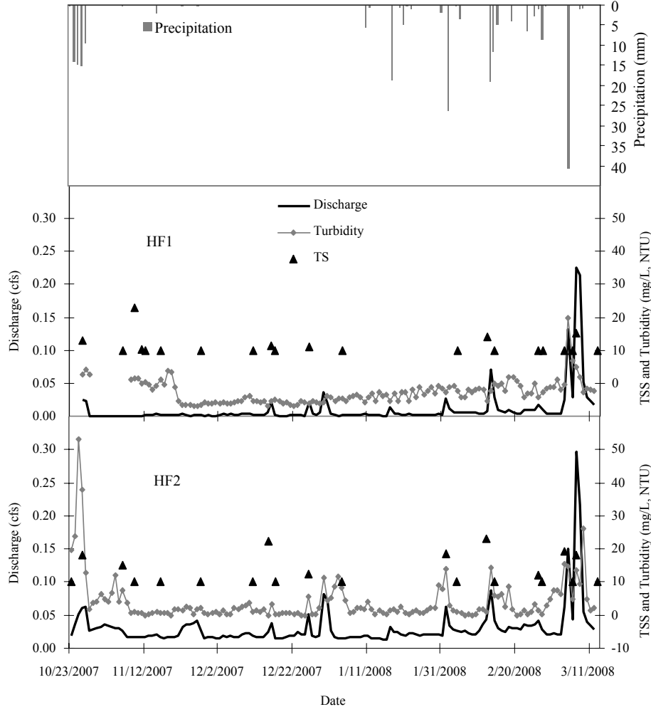
Figure 4. Daily precipitation, stream flow, turbidity and total suspended solids (TSS) patterns during calibration period for paired watersheds HF1 and HF2, Hill Forest.
