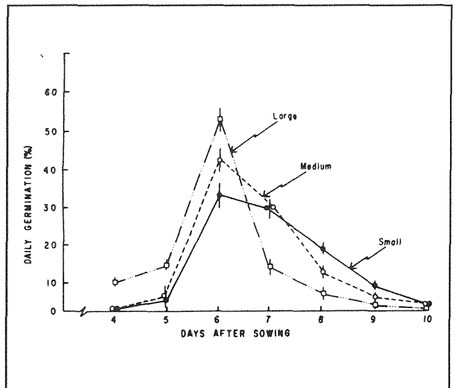
Fig. 2. Mean daily germination of loblolly pine seeds from the large, medium, and small classes incubated under standard laboratory conditions (from Dunlap and Barnett 1983). Vertical bar represent one SE.
