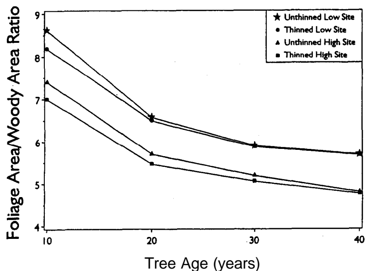
Figure 17.9. Trends over time of the ratio of predicted foliage surface area to predicted woody tissue surface area of an example codominant-dominant loblolly pine tree in stands of two site indices either thinned or unthinned.
