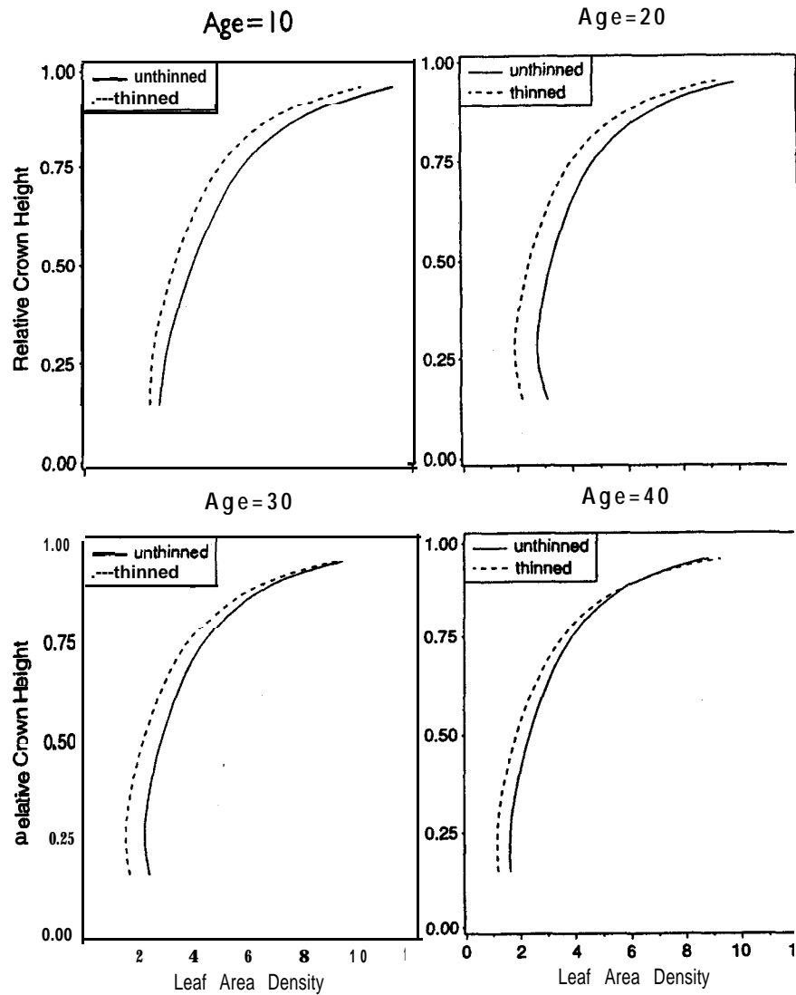
Figure 17.6. Predicted leaf area density for various relative crown heights at ages 10, 20, 30, and 40 of an example codominant-dominant loblolly pine tree in thinned or unthinned stands of site index equalling 21.3 m.
