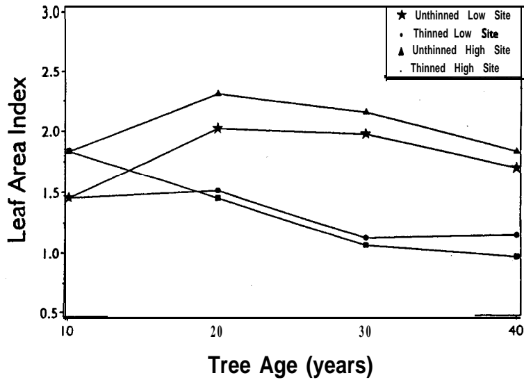
Figure 17.4. Predicted trends in stand leaf area index through time in loblolly pine stands of two site indices either thinned or unthinned.
