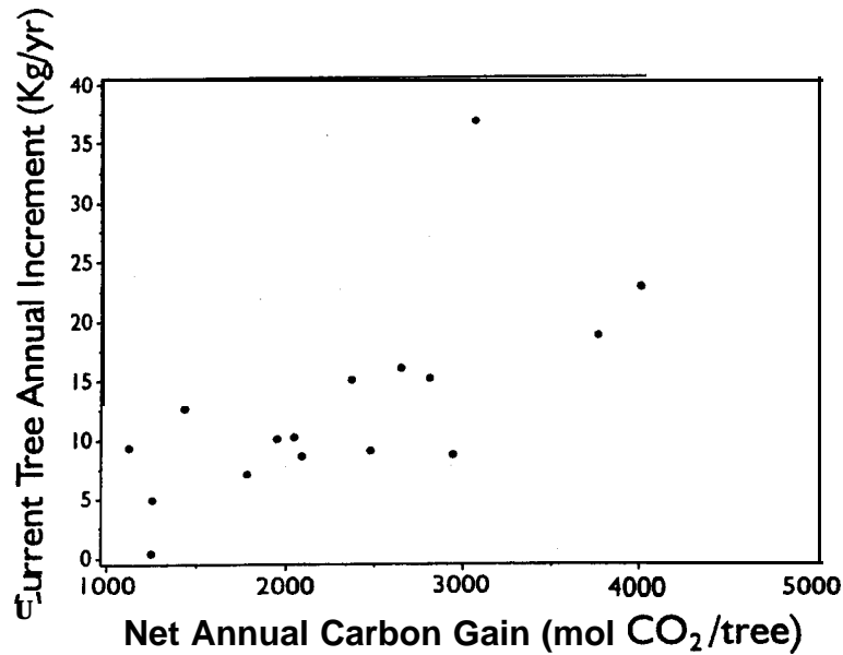
Figure 17.12. Predicted present-day annual woody biomass yield compared to predicted net annual carbon gain at ages ten, twenty, thirty, and forty for an example codominant-dominant loblolly pine tree in stands of two site indices either thinned or unthinned.
