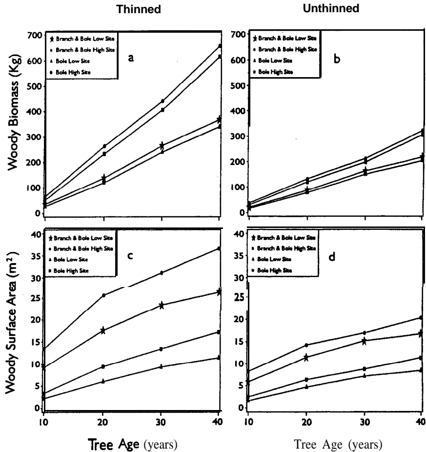
Figure 17.7. Comparison of predicted woody tissue weight and predicted surface area over time of an example codominant-dominant loblolly pine tree in stands of two site indices either thinned or unthinned.
