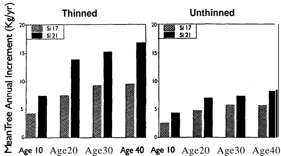
Figure 17.11. Trends of predicted mean annual woody biomass increment for an example codominant-dominant loblolly pine tree in stands of two site indices either thinned or unthinned
