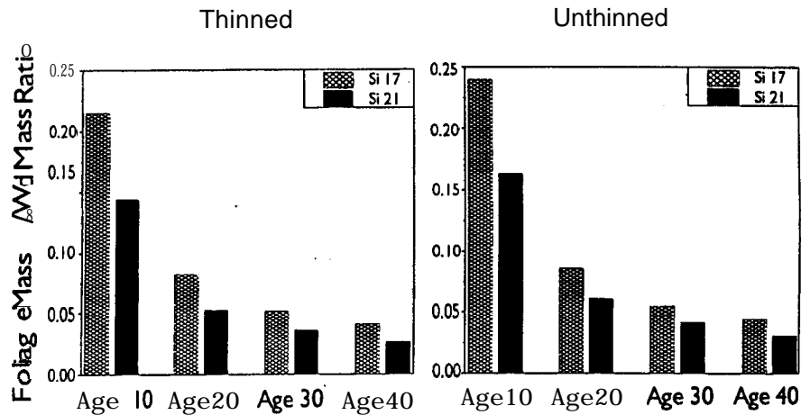
Figure 17.8. Trends over time of the ratio of predicted foliage biomass to predicted woody tissue biomass of an example codominant-dominant loblolly pine tree in stands of two site indices either thinned or unthinned.
