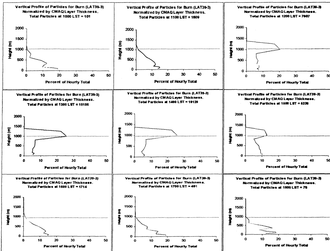
Fig. 3. Hourly vertical profiles of smoke developed by DAYSMOKE for the duration of a southern prescribed burn. Horizontal blue line identifies the top of the mixed layer (held constant for this simulation).
