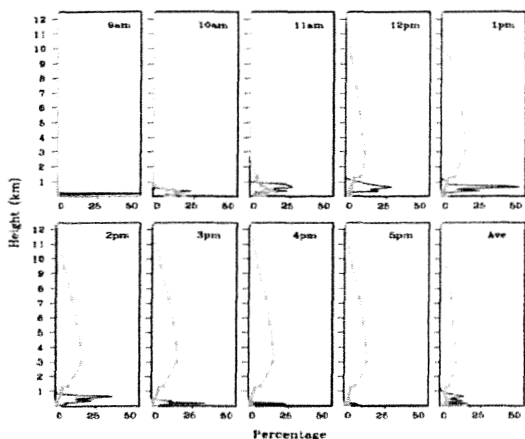
Fig. 5. Vertical distribution of smoke particles estimated using DAYSMOKE (pink) and Briggs scheme (green) on March 6, 2002.
