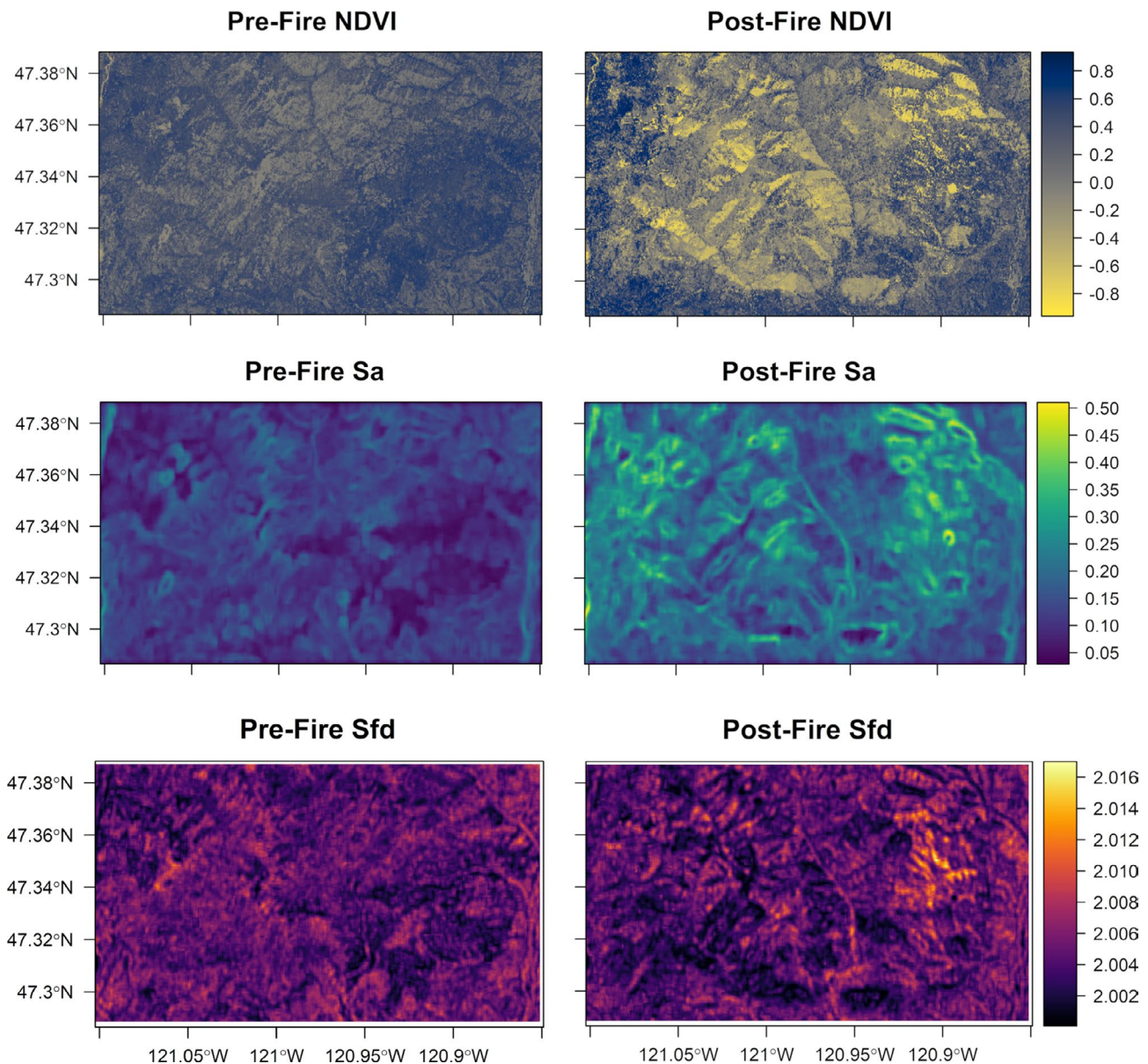
FIGURE 1 Pre- and post-fire Normalized Difference Vegetation Index (NDVI) for the 2017 Jolly Mountain fire in Washington (top panel), and texture images of average roughness ( S_a ; middle panel) and fractal dimension ( S_{fd} ; bottom panel) created from NDVI. Texture images were created using 30 \times 30 pixel ( 450 \text{ m} \times 450 \text{ m} ) square windows
