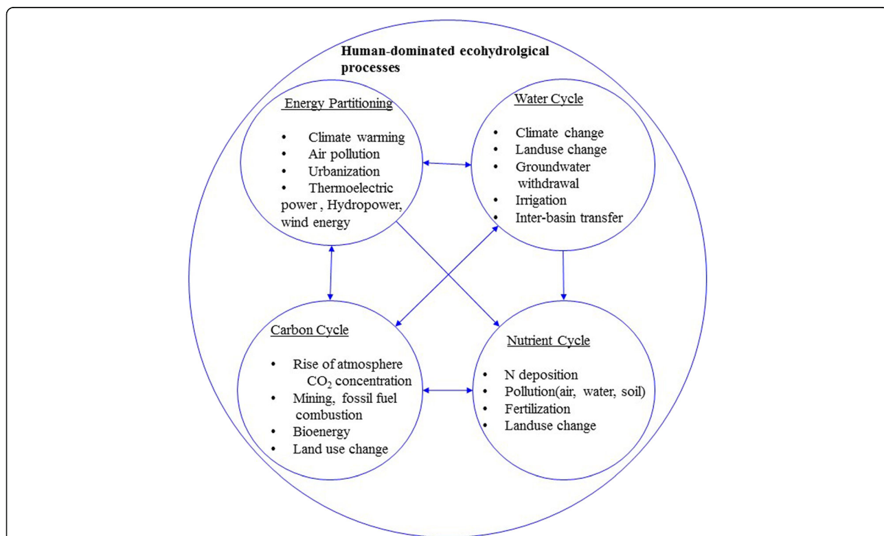
Fig. 2 A schematic overview of the inter-connected ecohydrological processes in human-dominated ecosystems. Human activities in the Anthropocene have permanently altered all aspects of the natural energy, water, carbon, and nutrient cycles by influencing the energy and material inputs to the biosphere, the hydrosphere, and the atmosphere
