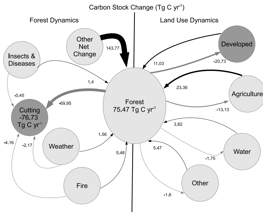
Figure 2 | Forest carbon stock changes (Tg C yr -1 ) resulting from land use dynamics (right side) and forest dynamics within forest land uses (left side). Line thickness is proportional to the flow. Standard errors are available in Tables S3 and S4.
