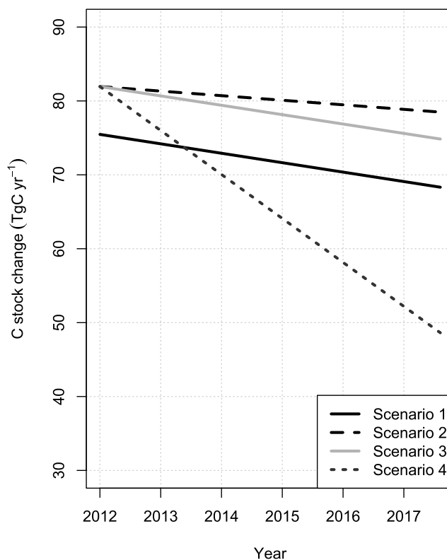
Figure 4 | Forest C stock change ( \text{Tg C yr}^{-1} ) from 2012 to 2017 based on integrated land use – forest age structure model. Scenario 1: forest remaining as forest from 2007–2012 projected to 2017. Scenario 2: Forest remaining as forest from 2012–2017 plus additions to forest land from other land uses. Land use transitions to forest were assumed to occur at the 2007–2012 rates. Scenario 3: Forest remaining as forest from 2012–2017 plus additions to forest land from other land uses. The 2007–2012 land use transition rates for agriculture to forest were decreased by 10% and the transitions from forest to developed were increased by 10%. All other rates remained at observed levels. Scenario 4: Forest remaining as forest from 2012–2017 plus additions to forest land from other land uses. The 2007–2012 land use transition rates for agriculture to forest were reversed.
