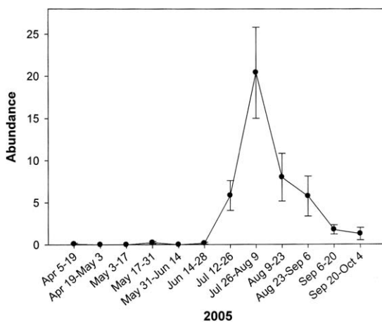
Fig. 1. Mean \pm SE ( n = 12 ) number of vespid wasps captured at twelve locations (canopy and ground traps combined) in a temperate deciduous forest.
