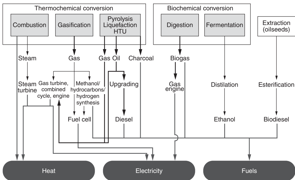
Fig. 20.7. Various thermochemical and biochemical conversion technologies for woody biomass and their various end-product scenarios (from Faaji, 2006).
