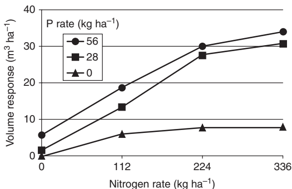
Fig. 20.4. Eight-year volume responses of loblolly pine to N and P fertilization (age 9–16 years) in the southern USA (adapted from Fox et al. , 2007).
