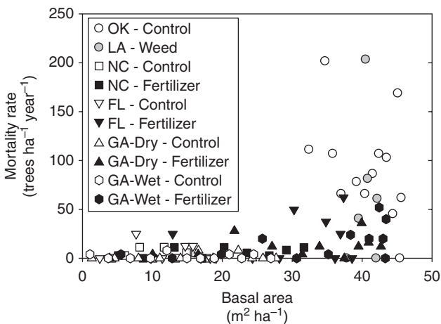
Fig. 20.3. Mortality rate of unthinned loblolly pine stands in relation to stand basal area (adapted from Jokela et al. , 2004).
