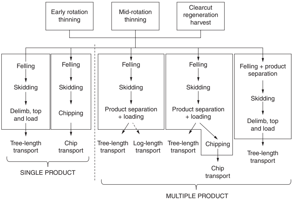
Fig. 20.5. Alternative harvesting systems for plantation pine and energy-wood.
