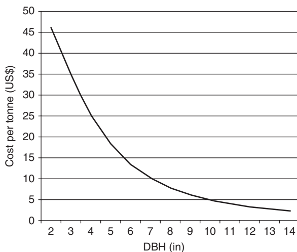
Fig. 20.6. Example felling cost function illustrating the effect of piece size on cost per tonne. DBH, diameter at breast height.
