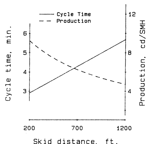
Figure 2.--Time per cycle in minutes and production per scheduled machine hour (SMH) as a function of skid distance.
